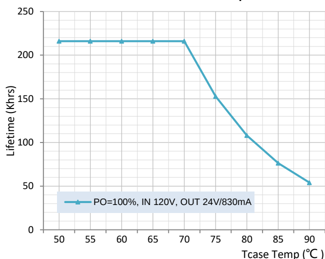
Lifetime vs. Tcase Temp
