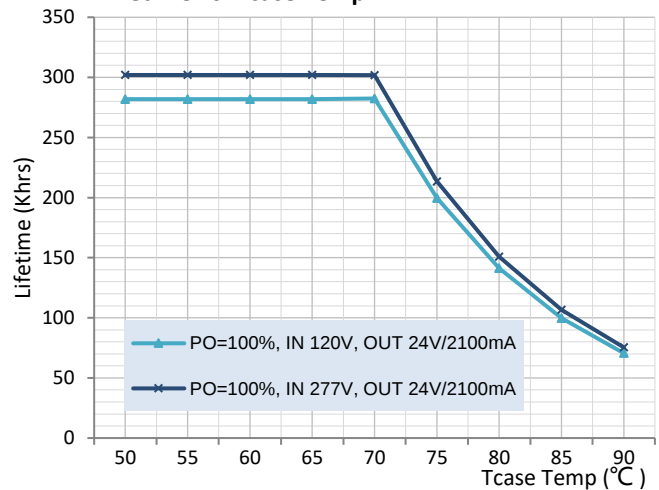
Lifetime vs. Tcase Temp
