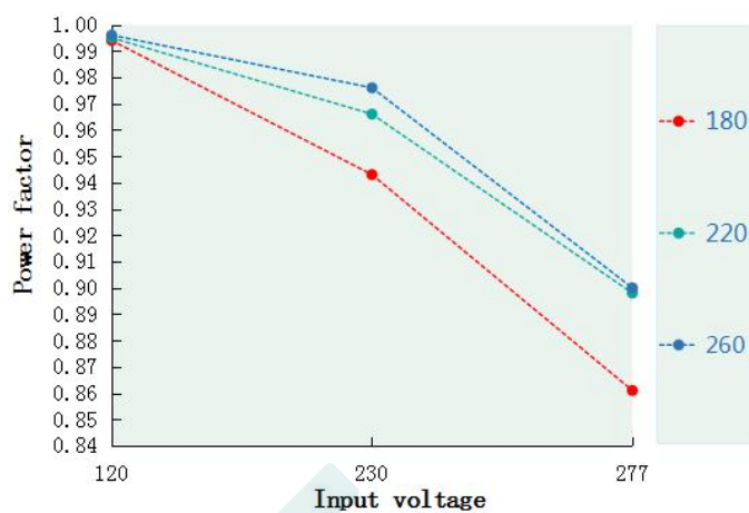
Power factor VS Input (DL-125W-V260A/S/X -SPF)
