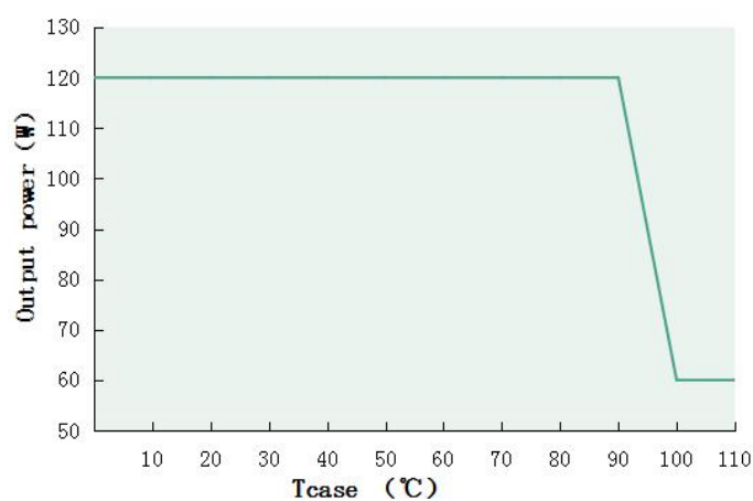
Output power VS Tcase (DL-125W-V260A/S/X -SPF)
