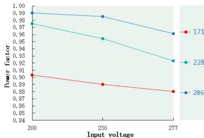
Power factor VS Input voltage(DL-200H-286A/P-MXC)
