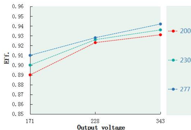
Eff. VS Output voltage(DL-200H-286A/P-MXC)
