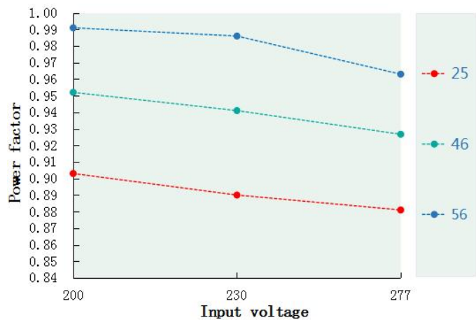
Power factor VS Input voltage(DL-200H-56A/P-MXC)
