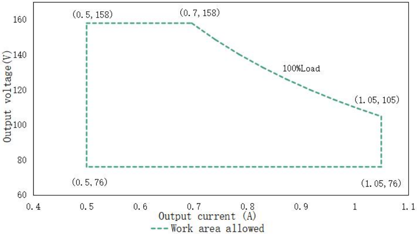
Output voltage VS output current of DL-110H-V158P/X-MXK (input: 200-277Vac)
