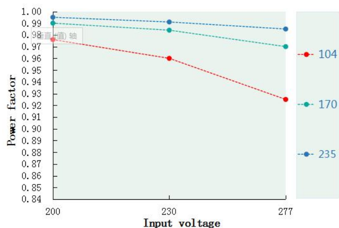
Power factor VS Input voltage(DL-165H-V235P/X-MXK)
