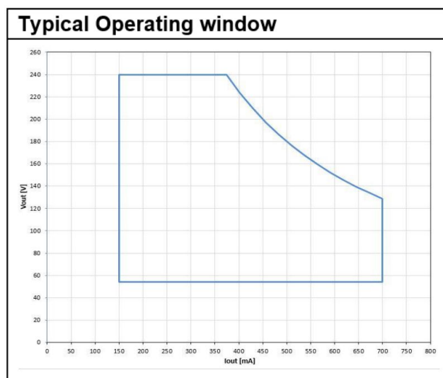
OTI DALI 90/220-240/700 D LT2 L Operating Window
