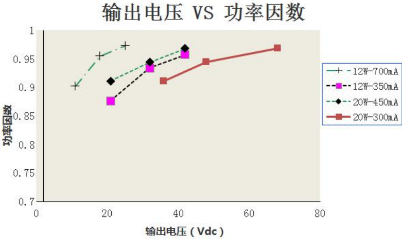
Vout VS PF
