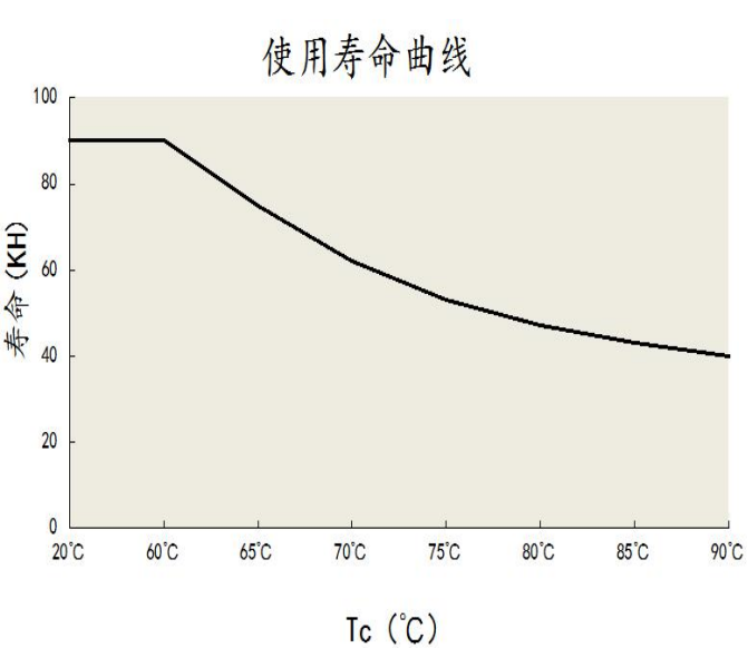
Tc VS Life
