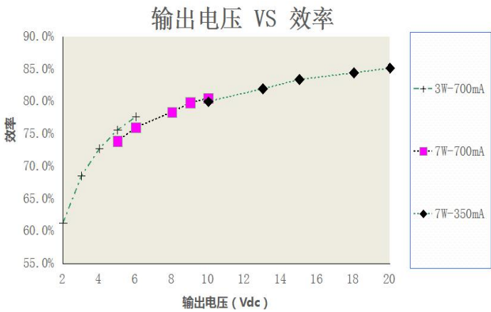
Vout VS Efficiency
