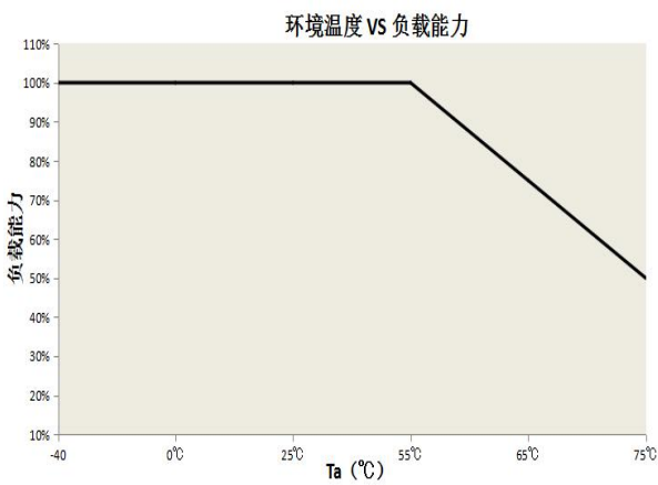
Load reduction curve
