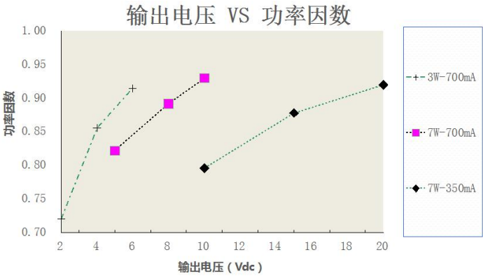
Vout VS PF
