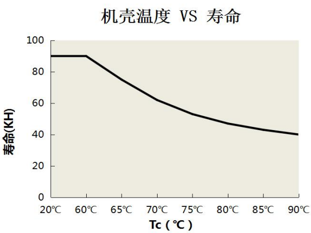
Tc VS Life
