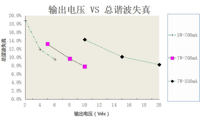
Vout VS THD
