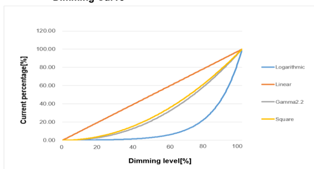
▪ Dimming Curve
