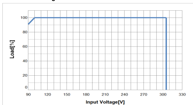
▪ Derating Curve
