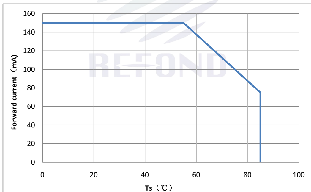
Fig.4-Solder Temperature Vs Forward Current 管脚温度与正向电流特性曲线
