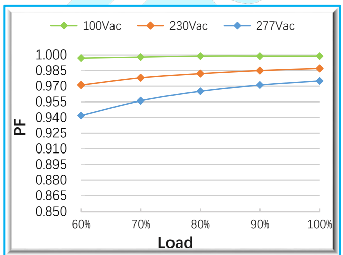
◇ PF Vs. Pout
