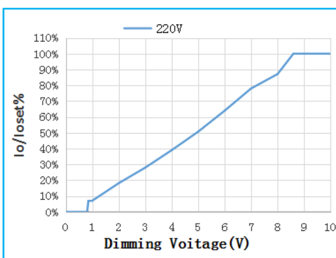
◇ I o /I o set vs. Dimming Voltage
