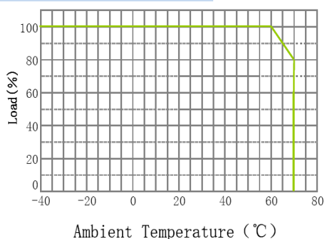
Derating Curve
