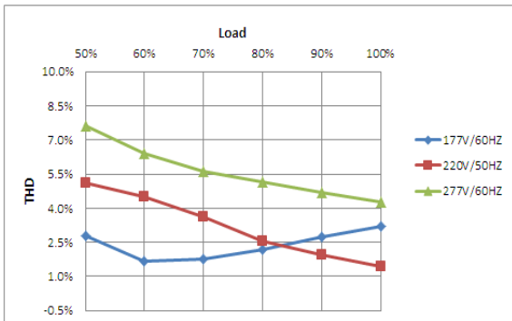
THD Curve
