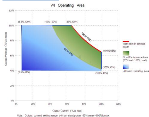
V/I Curve
