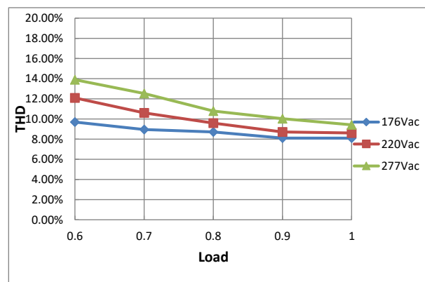
THD Curve
