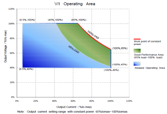
V/I Curve
