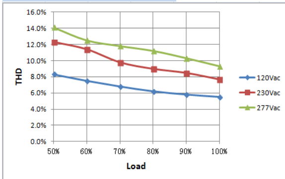
THD VS. Load Curve
