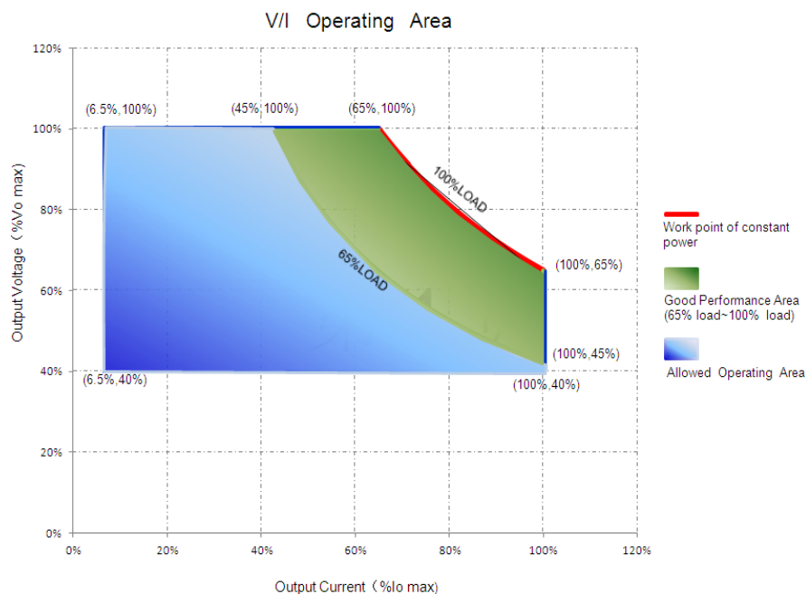
V/I Curve
