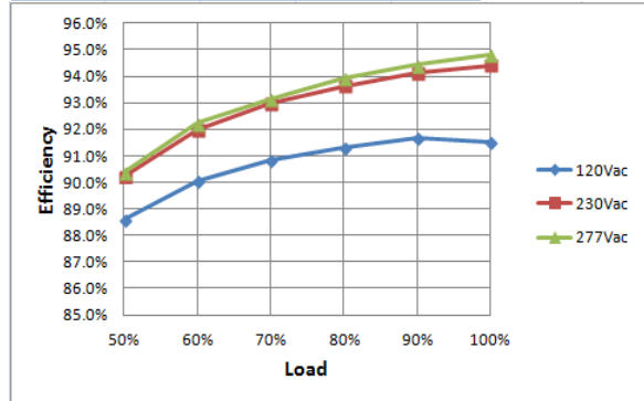
Efficiency VS. Load Curve (1300mA for Ref.)
