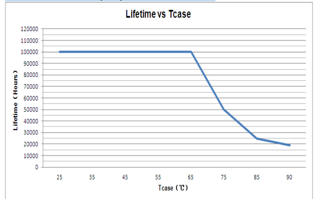
Life Time VS. Tcase (Ref.)
