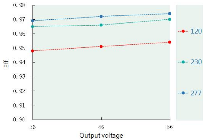
Eff. VS Output voltage(DL1000W-V56X-MXS)
