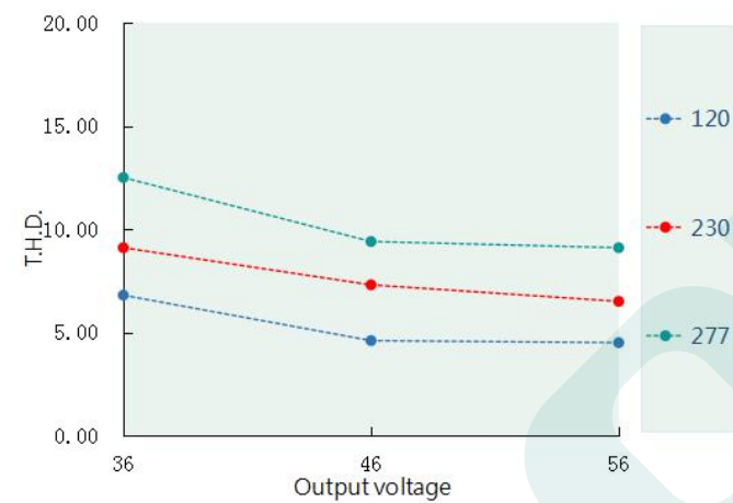
T.H.D. VS Output power(DL1000W-V56X-MXS)
