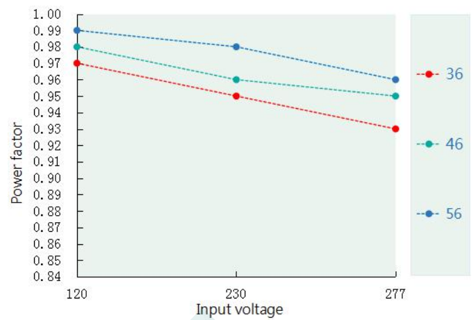
Power factor VS Input voltage(DL1000W-V56X-MXS)
