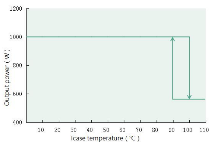
Output power VS Tcase (DL1000W-V56X-MXS)
