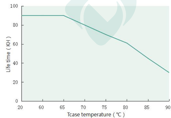
Tcase VS Lifetime(DL1000W-V56X-MXS)
