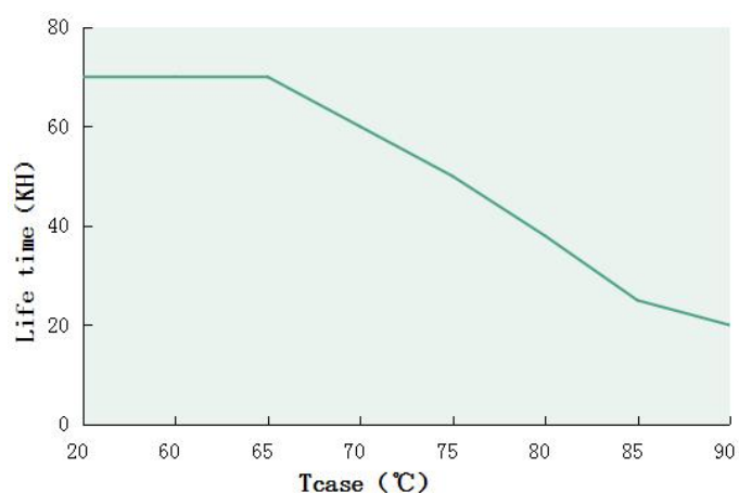
Tcase VS Lifetime(DL-75H-260P/A-PXC)
