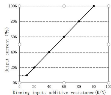
dimming curve
