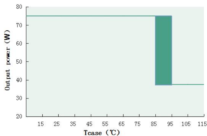
Output power VS Tcase (DL-75H-260P/A-PXC)
