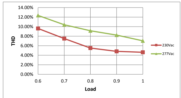
THD Curve
