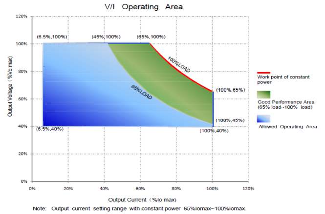
V/I Curve
