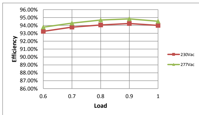
Efficiency VS. Load Curve (Io=700mA)
