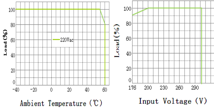
Derating Curve
