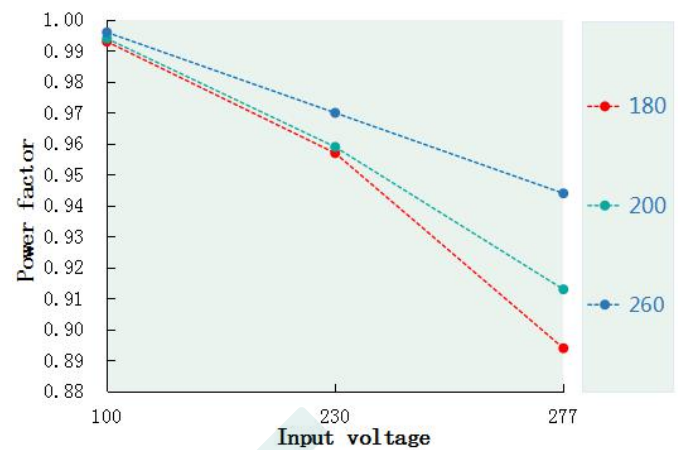
Power Factor VS Input Voltage (DL-200Z-260X -PXS)
