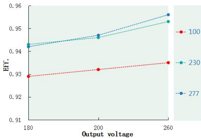
Eff. VS Output voltage (DL-200Z-260X -PXS)
