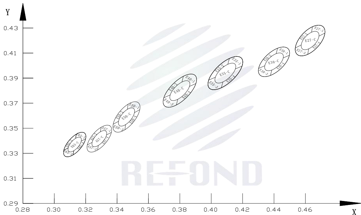
Fig 1-6-1 The C.I.E Chromaticity Diagram CIE色度图
