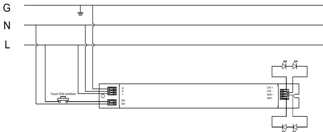
Fig.B:Push Dimming
