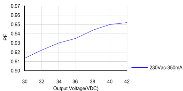
Power Factor Characteristics
