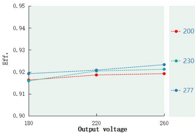
Eff. VS Output voltage(DL-50H-260P/A-PXC)
