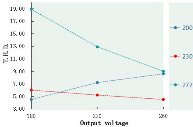
T.H.D. VS Output voltage(DL-50H-260P/A-PXC)
