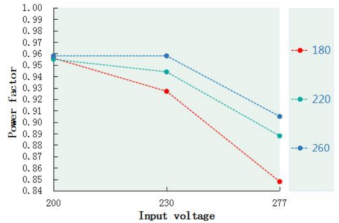
Power factor VS Input voltage(DL-50H-260P/A-PXC)
