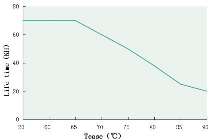
Tcase VS Lifetime(DL-50H-260P/A-PXC)
