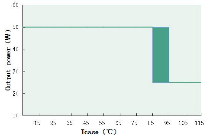
Output power VS Tcase (DL-50H-260P/A-PXC)
