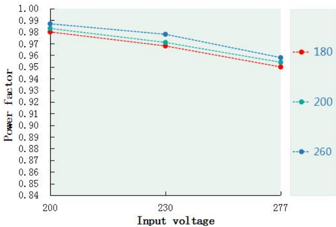
Power factor VS Input voltage(DL-240H-PXC)
