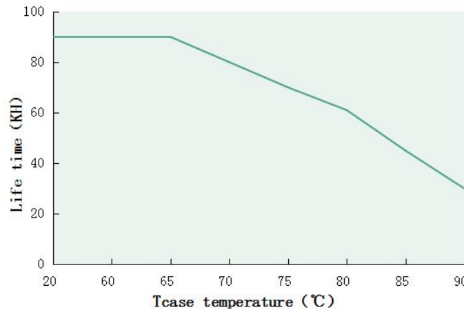
Tcase VS Lifetime(DL-240H-PXC)
