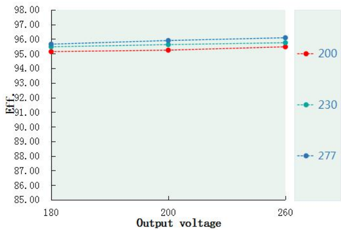
Eff. VS Output voltage(DL-240H-PXC)
