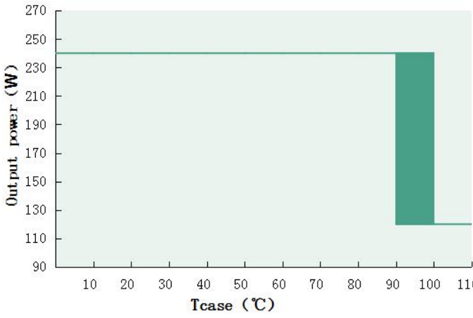
Output power VS Tcase(DL-240H-PXC)
