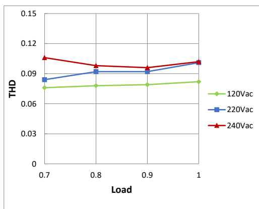
THD Curve
