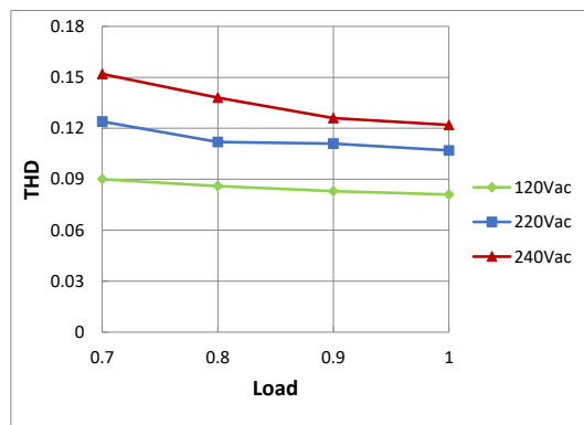
THD Curve
