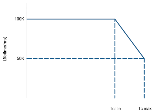
Lifetime vs. Temperature Curve
