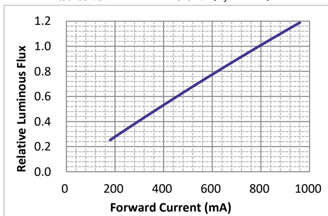
Relative luminous flux vs. forward current 相对亮度与正向电压曲线 ( T_j=25^{\circ}\text{C} )
