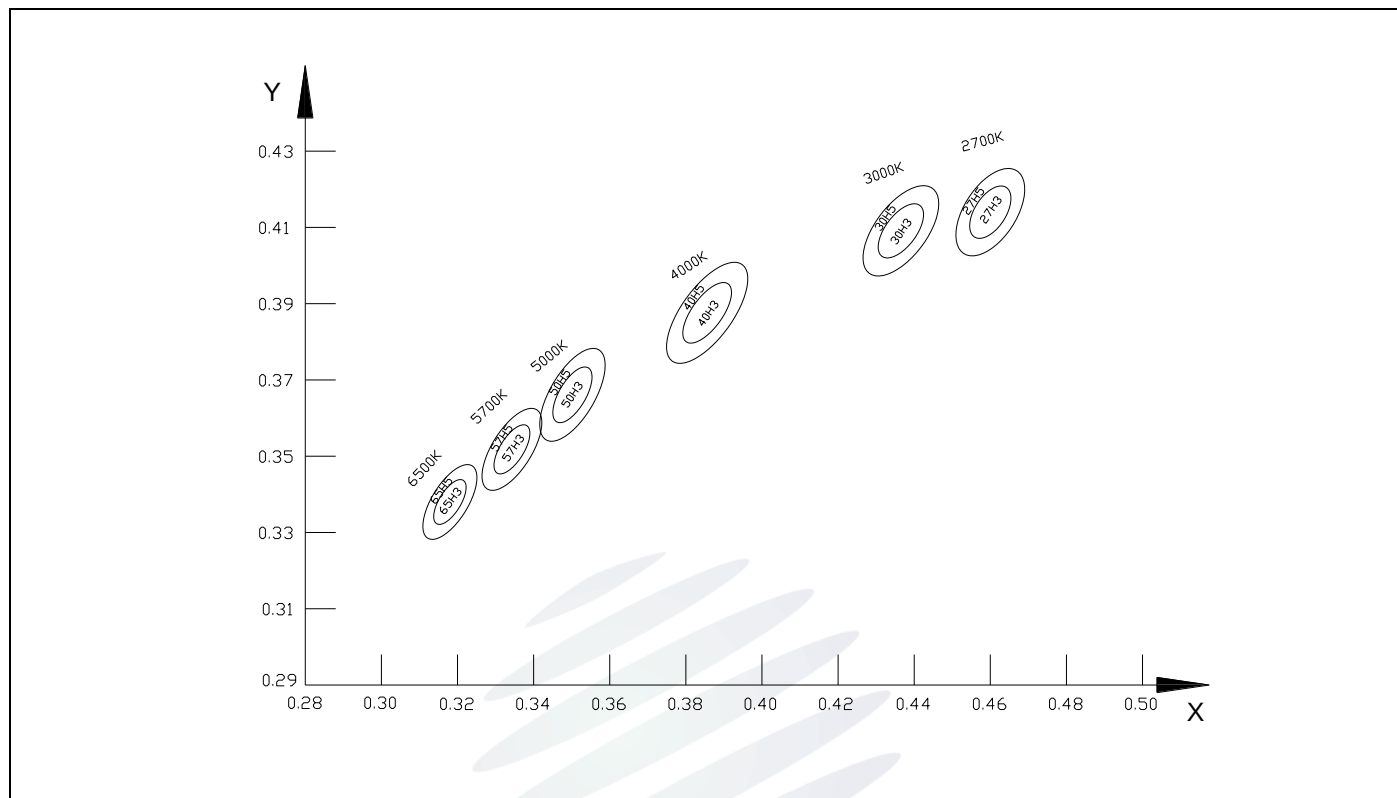
CIE 1931 chromaticity diagram
