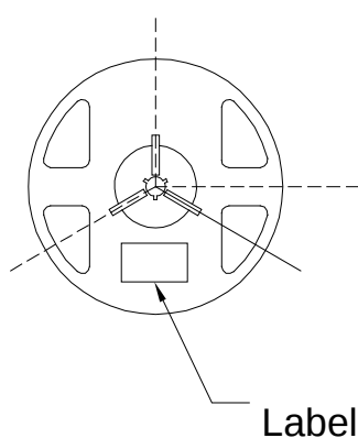
Fig.2-2 Reel 卷盘
