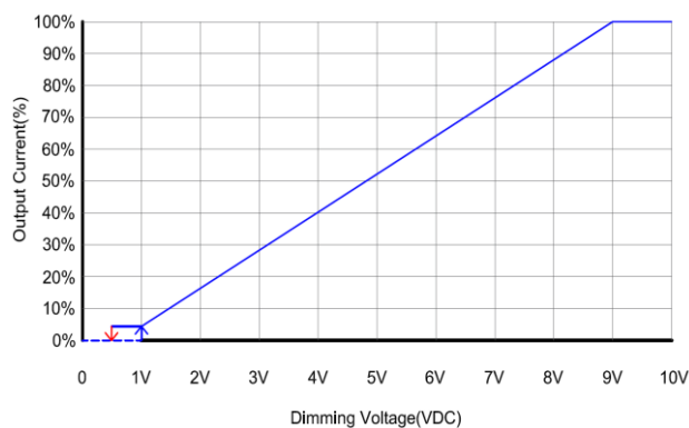
Dimming curve
