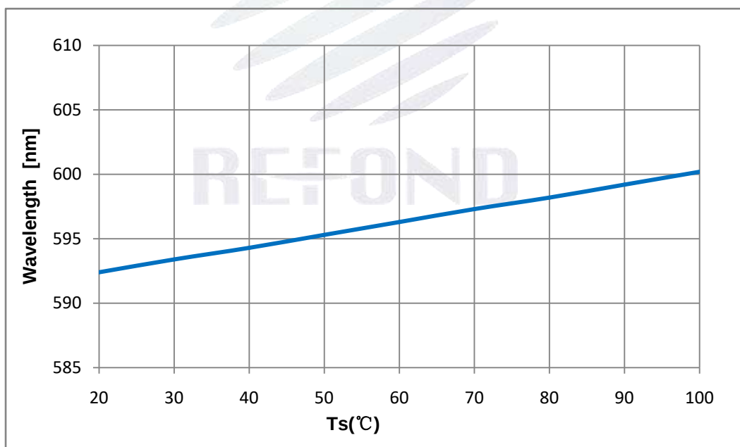
Fig 1-11 Wavelength Vs. Pin Temperature波长与引脚温度特性曲线
