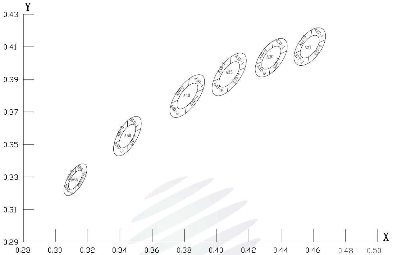
Fig 1-6 The C.I.E Chromaticity Diagram CIE色度
