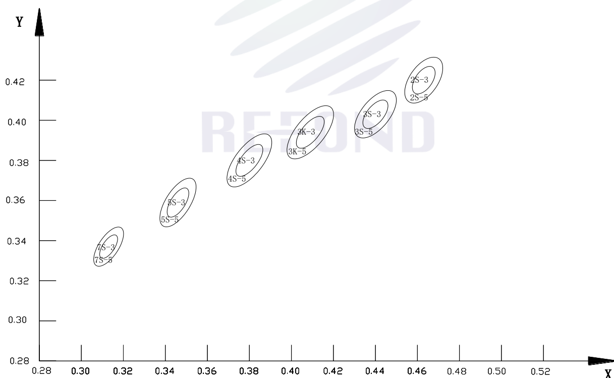
Fig 1-4 The C.I.E Chromaticity Diagram CIE 色度图
