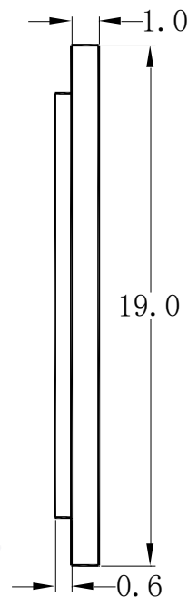
Fig.1-2 Side view 侧面视图
