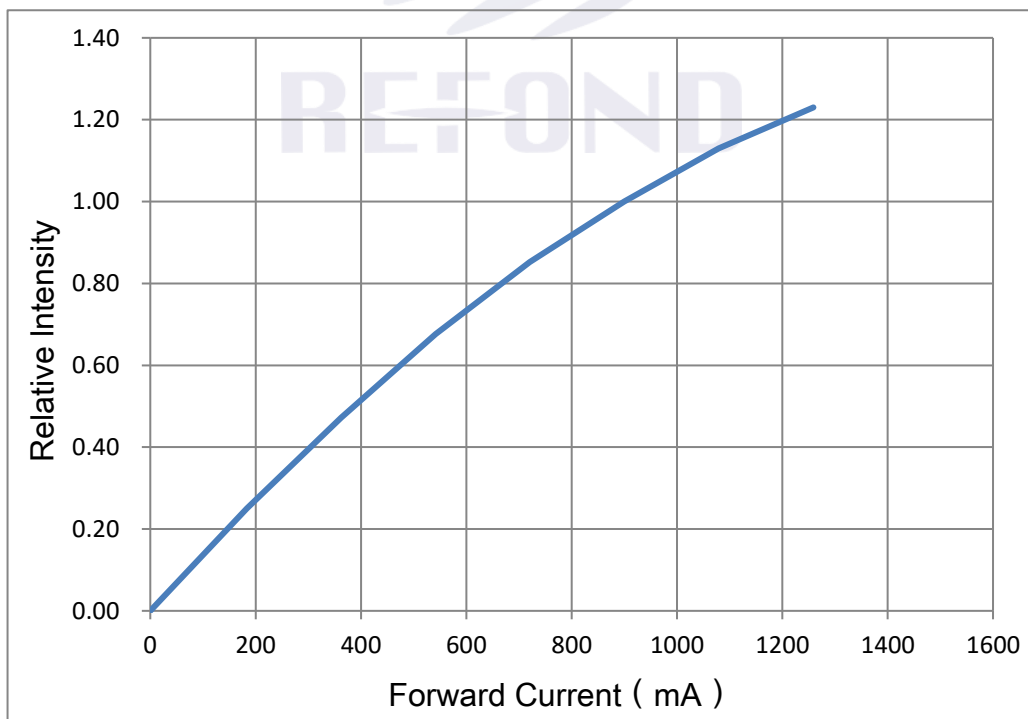
Fig 1-6 Forward Current Vs. Relative Intensity. 正向电流与相对光强特性曲线
