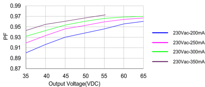
Power Factor Characteristics
