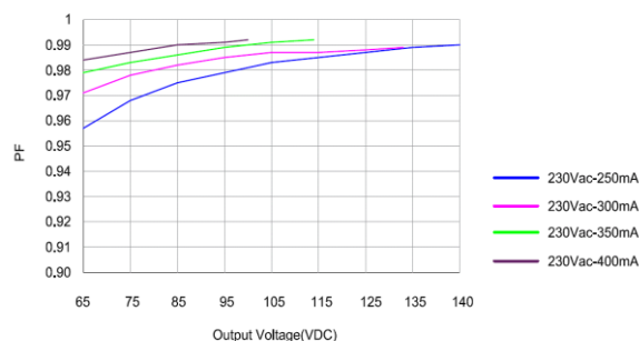
Power Factor Characteristics
