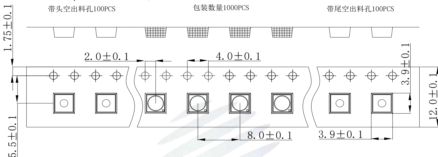
Fig.2-1 Carrier Tape Dimension 載帶尺寸
