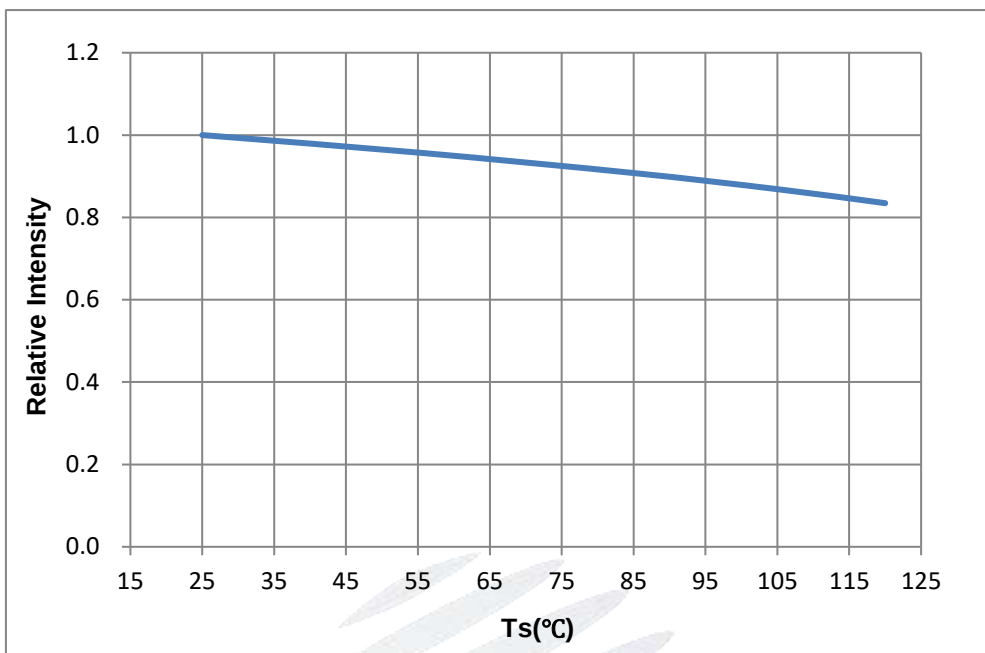
Fig.1-9 Temperature Vs Relative Intensity 引脚温度与相对光强特性曲线
