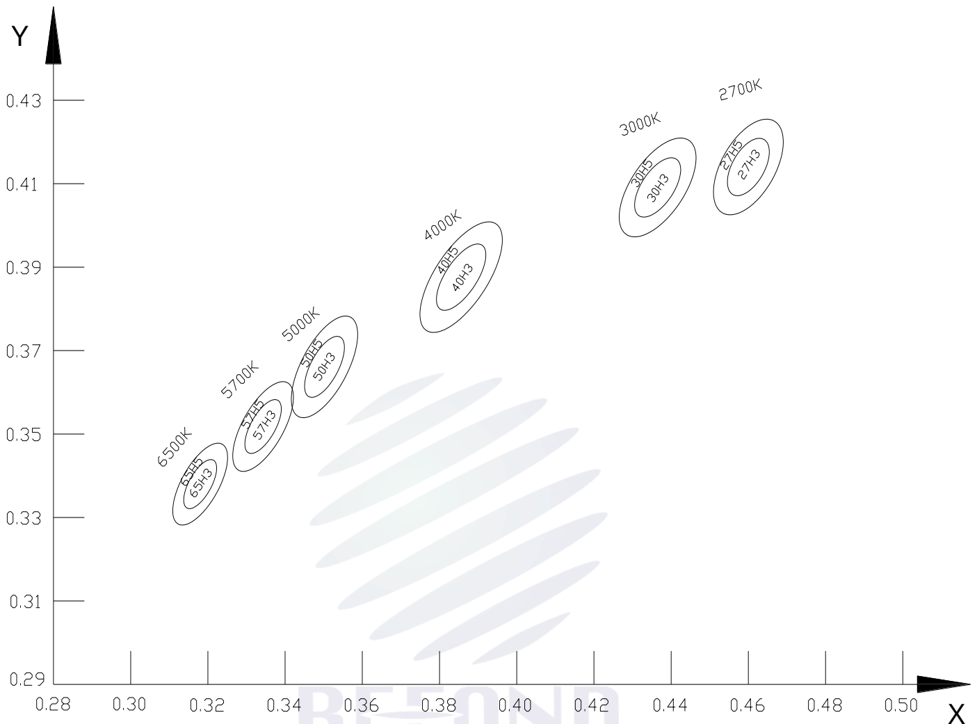
Fig 1-6 The C.I.E Chromaticity Diagram CIE色度图
