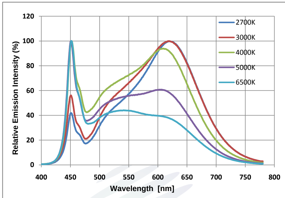
Fig 1-13 Spectrum Distribution光光谱分布特性曲线
