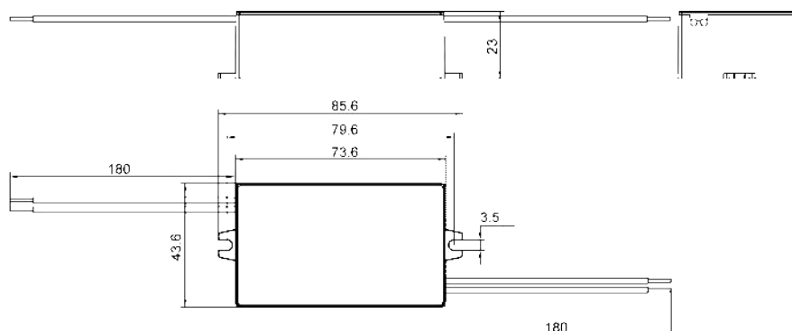
Dimension Drawing(mm)
