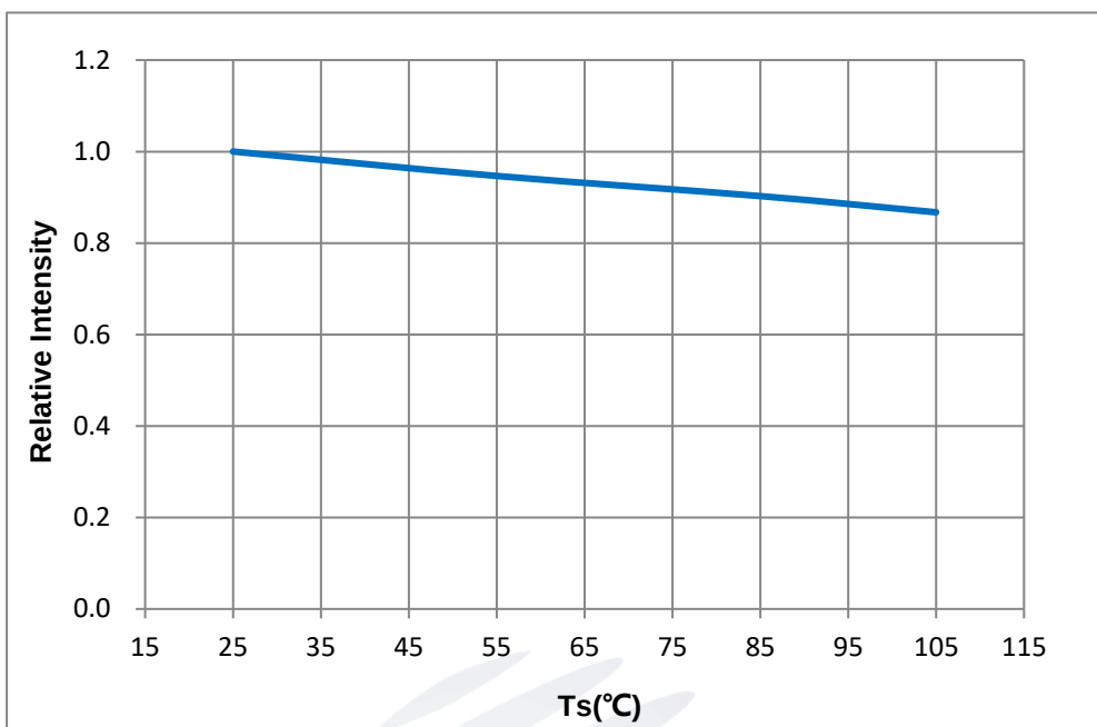
Fig.1-21 Temperature Vs Relative Intensity 引脚温度与相对光强特性曲线
