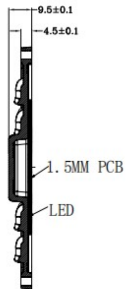
SECTION B—B
