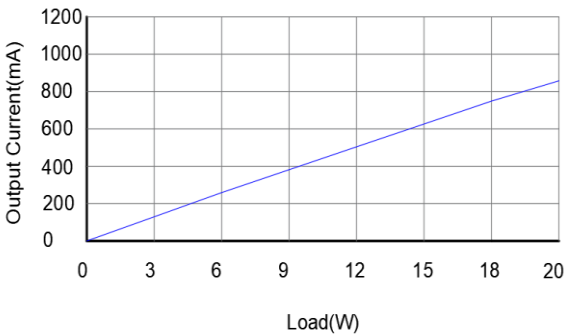
Output Current vs. Load
