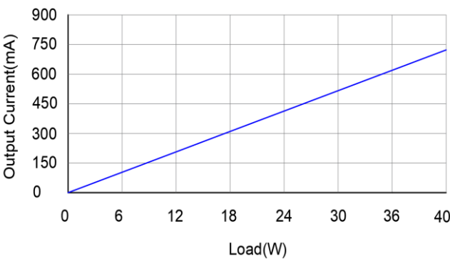
Output Current vs. Load
