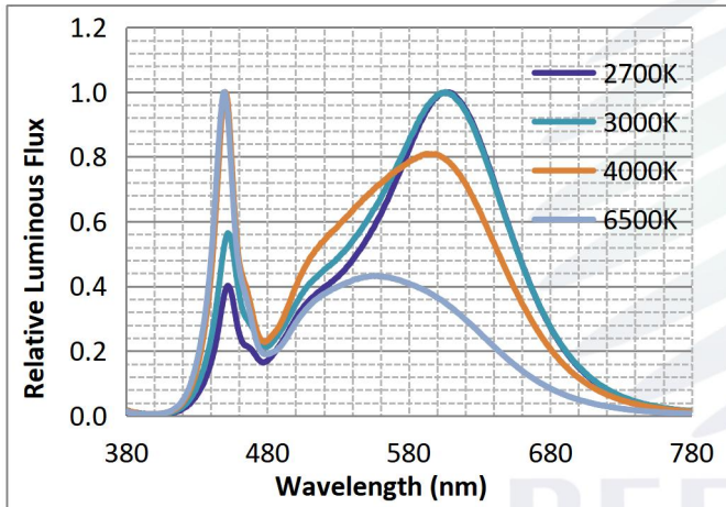
Typical spectrum distribution 典型光谱分布 ( T_s=25^\circ\text{C} IF=150mA)
