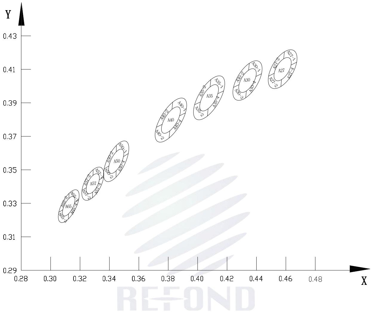
Fig 1-6 The C.I.E Chromaticity Diagram CIE色度
