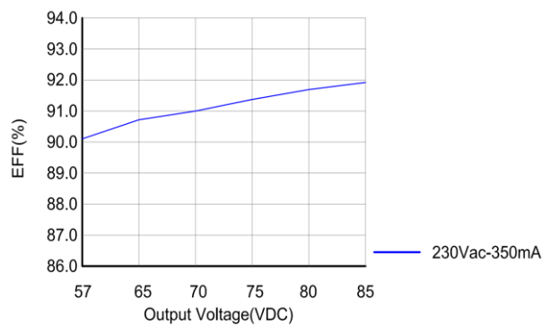
Efficiency VS.Load
