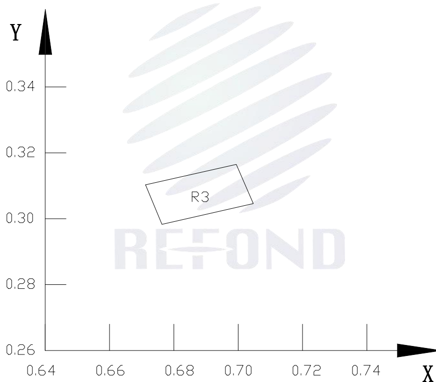
Fig 1-6 The C.I.E Chromaticity Diagram CIE色度图
