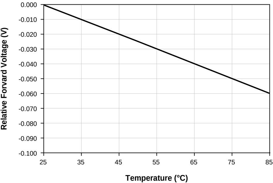
Fig 7. Junction Temperature vs. Relative Forward Voltage, I_F=150\text{mA}
