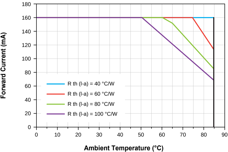
Fig 9. Ambient Temperature vs. Maximum Forward Current, T_{j\_max} = 125^{\circ}C
