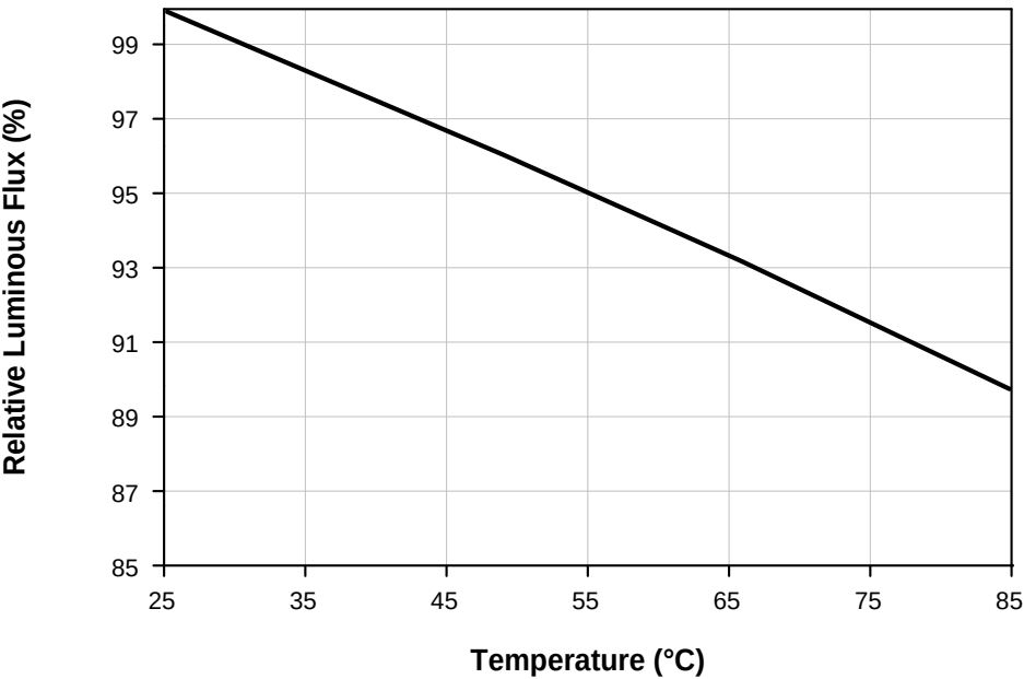
Fig 6. Junction Temperature vs. Relative Luminous Flux, I_F=150\text{mA}
