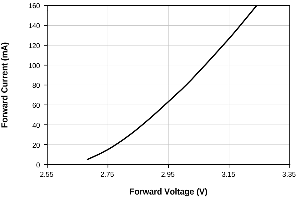
Fig 3. Forward Voltage vs. Forward Current, T_j = 25^{\circ}\text{C}
