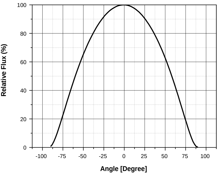
Fig 2. Radiant Pattern, T_j = 25^{\circ}\text{C} , I_F=150\text{mA}
