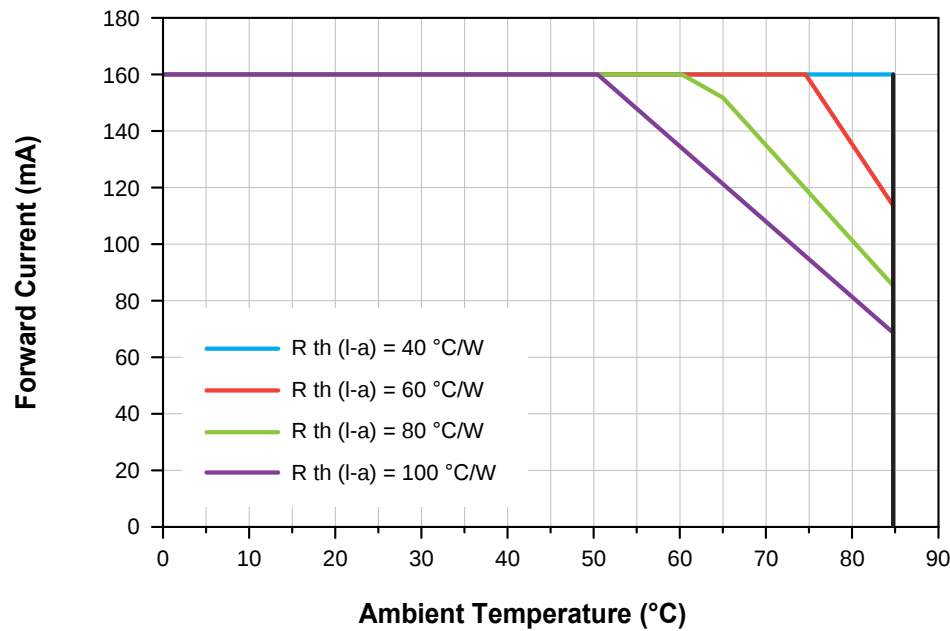
Fig 9. Ambient Temperature vs. Maximum Forward Current, T_{j\_max} = 125^{\circ}\text{C}
